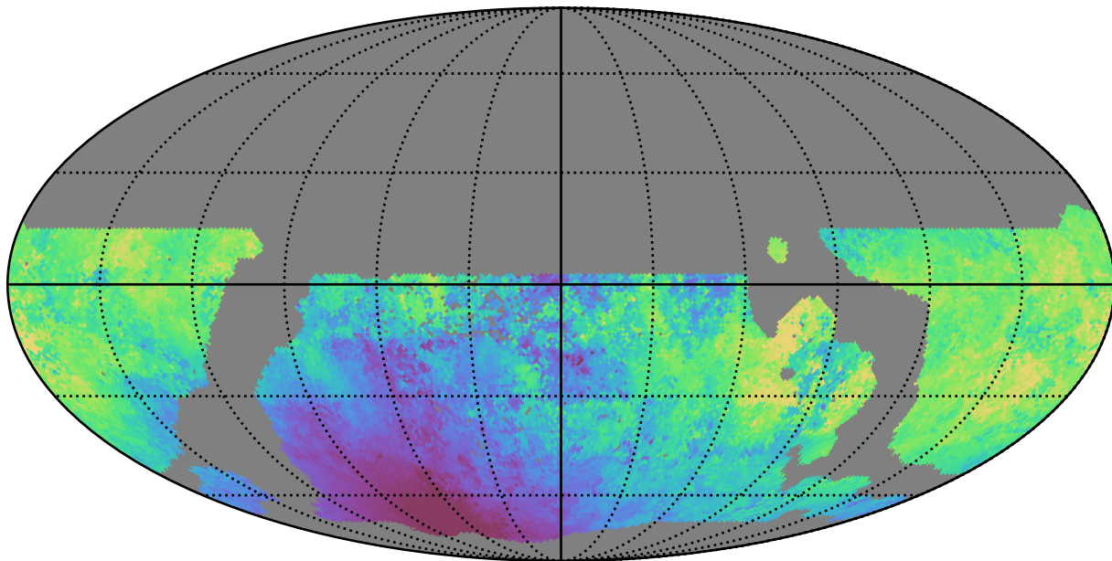
weather_cloudso30v3.4_10yrs WFD u band: Median moonDistance
