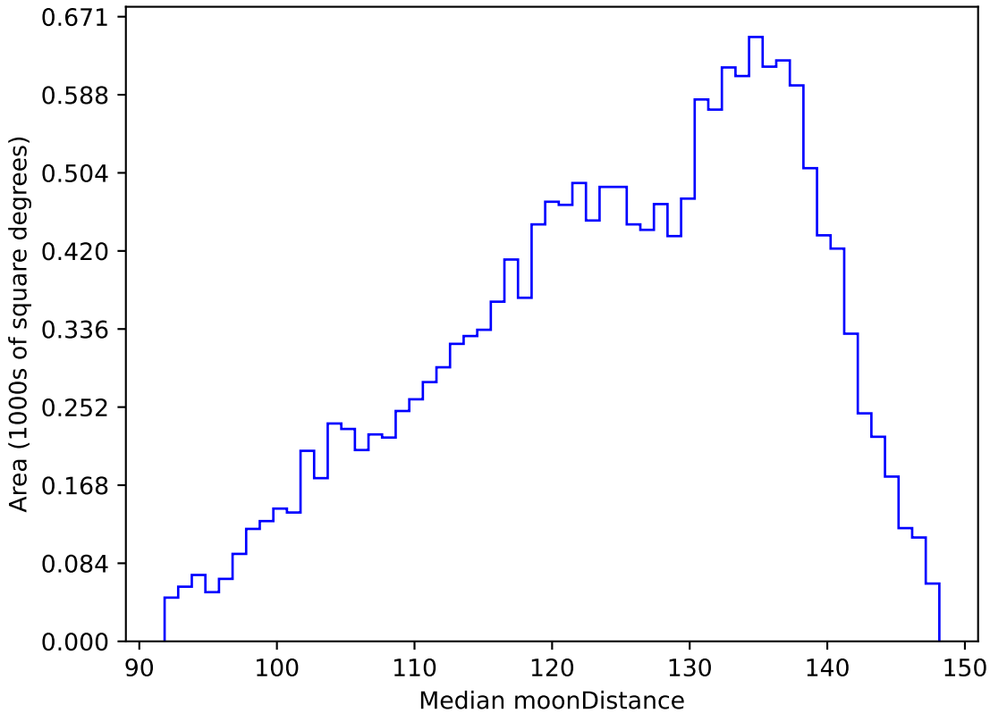
weather_cloudso30v3.4_10yrs WFD u band: Median moonDistance
