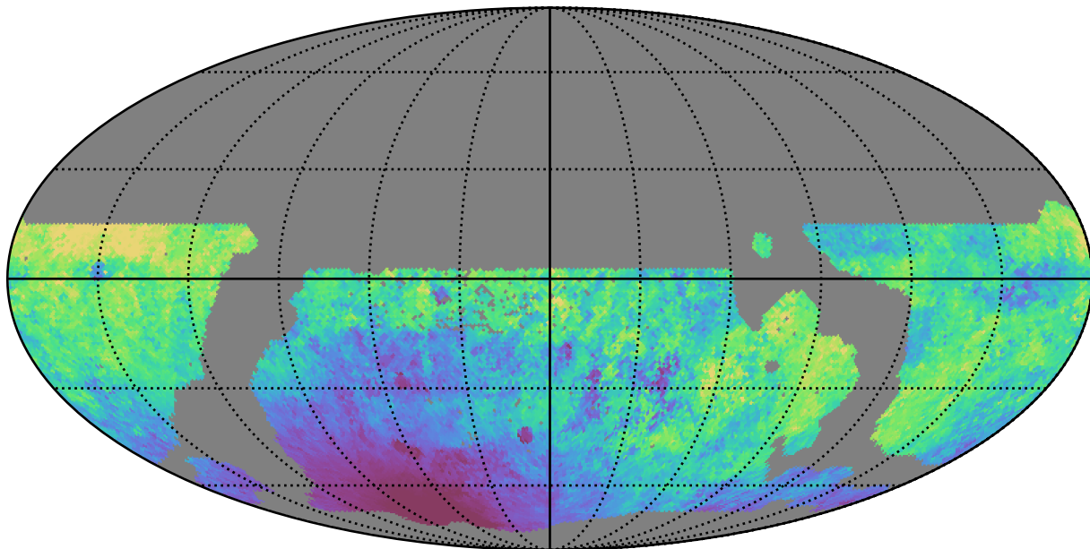
weather_cloudso30v3.4_10yrs WFD r band: Median moonDistance
