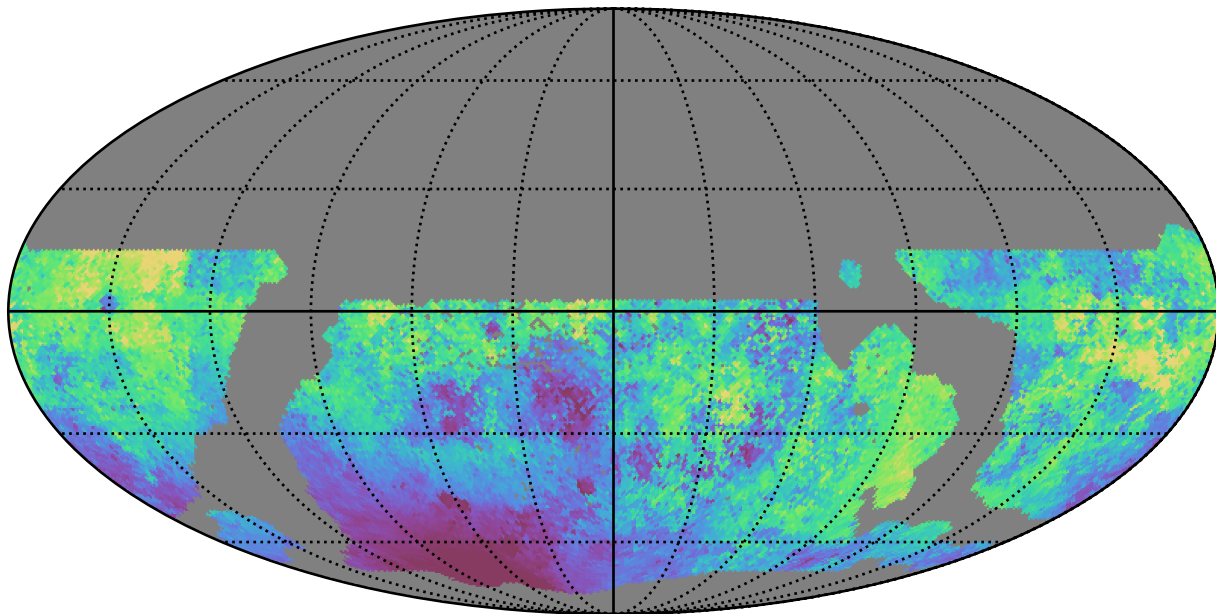
weather_cloudso30v3.4_10yrs WFD g band: Median moonDistance
