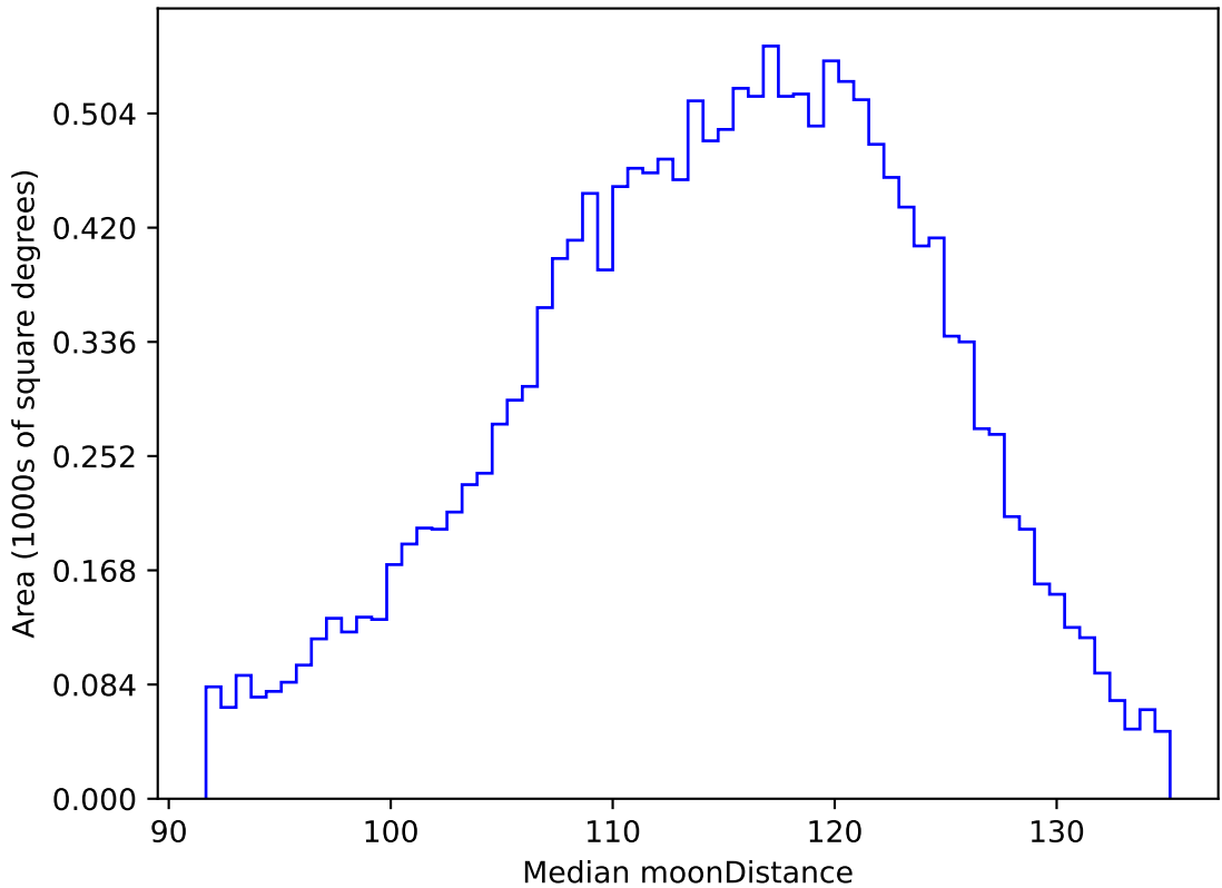
weather_cloudso30v3.4_10yrs WFD g band: Median moonDistance
