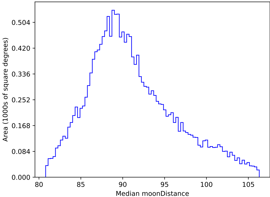
weather_cloudso30v3.4_10yrs WFD all bands: Median moonDistance
