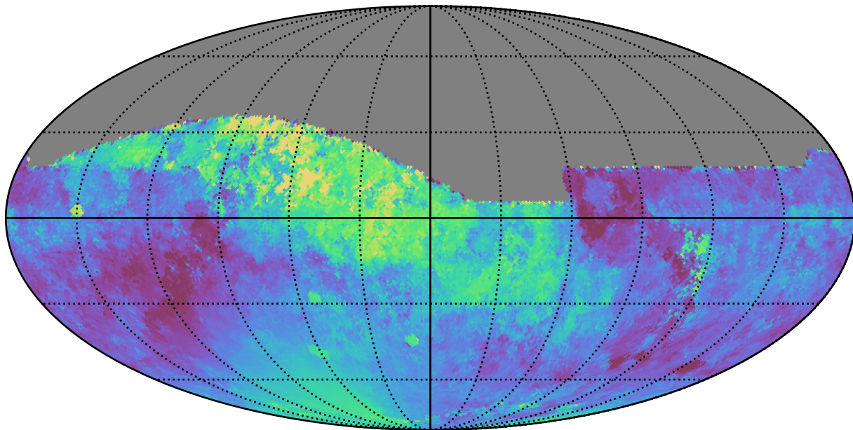
weather_cloudso30v3.4_10yrs All sky z band: Median moonDistance
