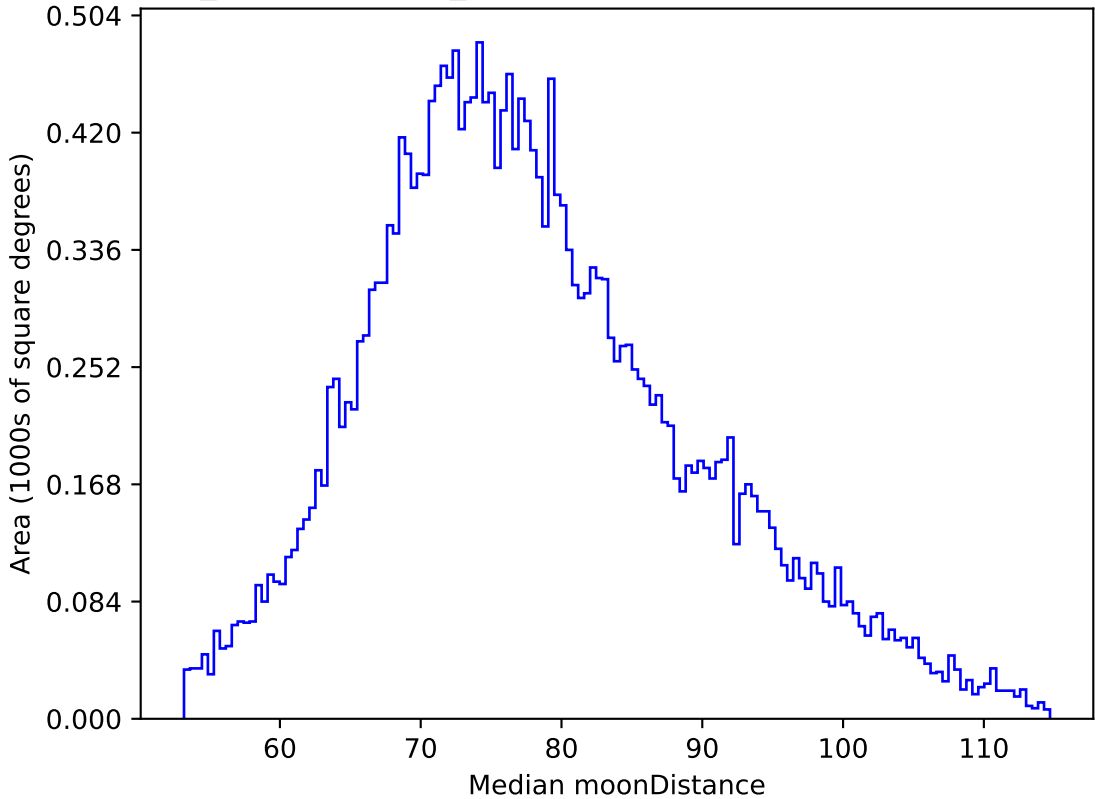
weather_cloudso30v3.4_10yrs All sky z band: Median moonDistance
