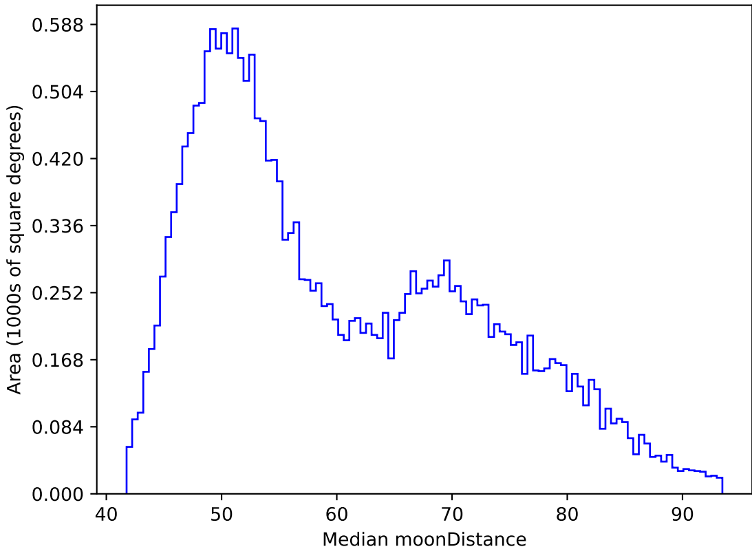
weather_cloudso30v3.4_10yrs All sky y band: Median moonDistance
