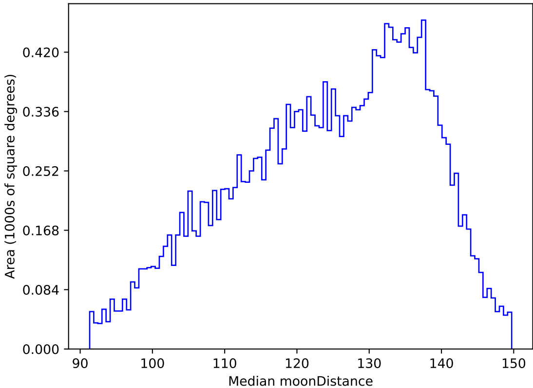
weather_cloudso30v3.4_10yrs All sky u band: Median moonDistance
