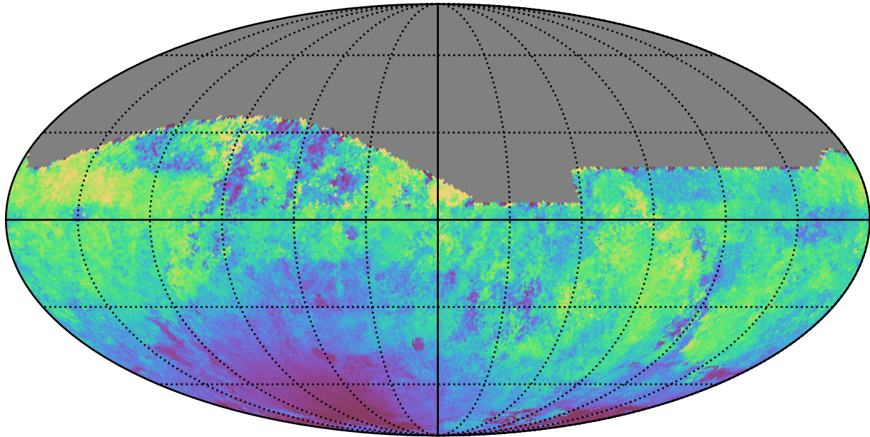
weather_cloudso30v3.4_10yrs All sky r band: Median moonDistance
