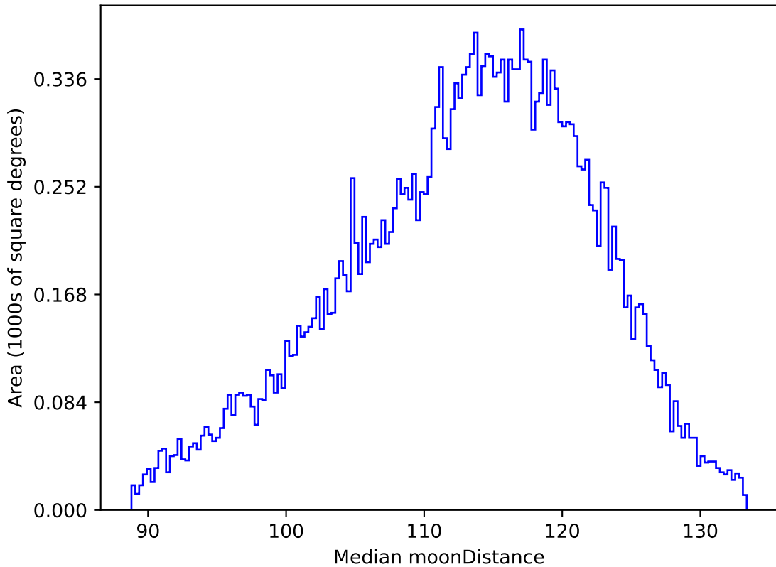
weather_cloudso30v3.4_10yrs All sky r band: Median moonDistance
