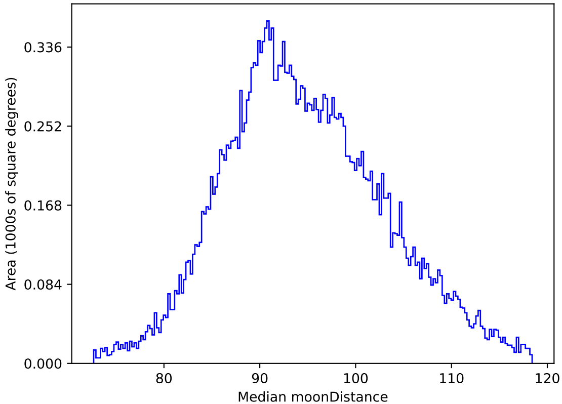
weather_cloudso30v3.4_10yrs All sky i band: Median moonDistance
