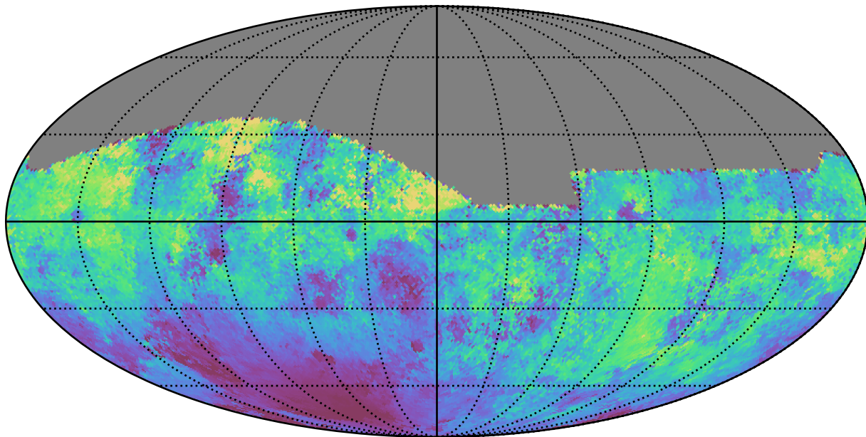
weather_cloudso30v3.4_10yrs All sky g band: Median moonDistance
