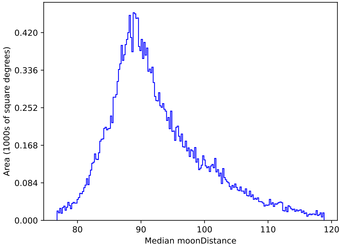
weather_cloudso30v3.4_10yrs All sky all bands: Median moonDistance
