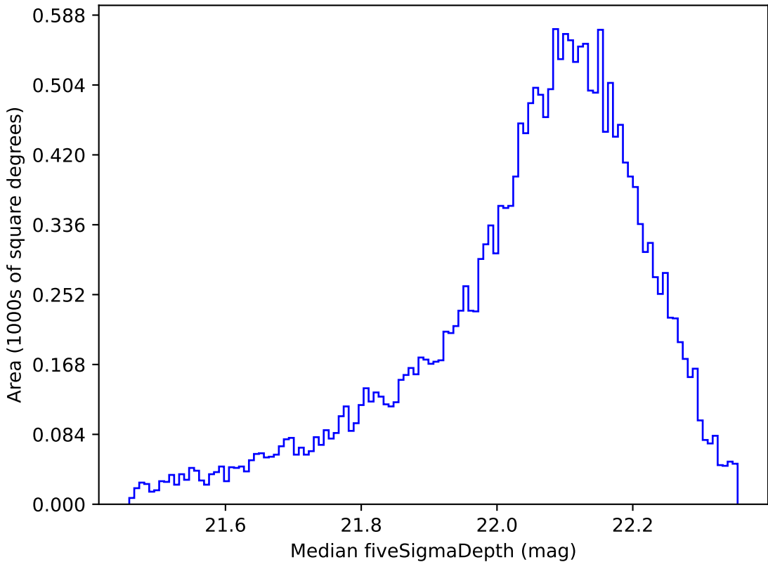
weather_cloudso30v3.4_10yrs Yr 1 y band: Median fiveSigmaDepth
