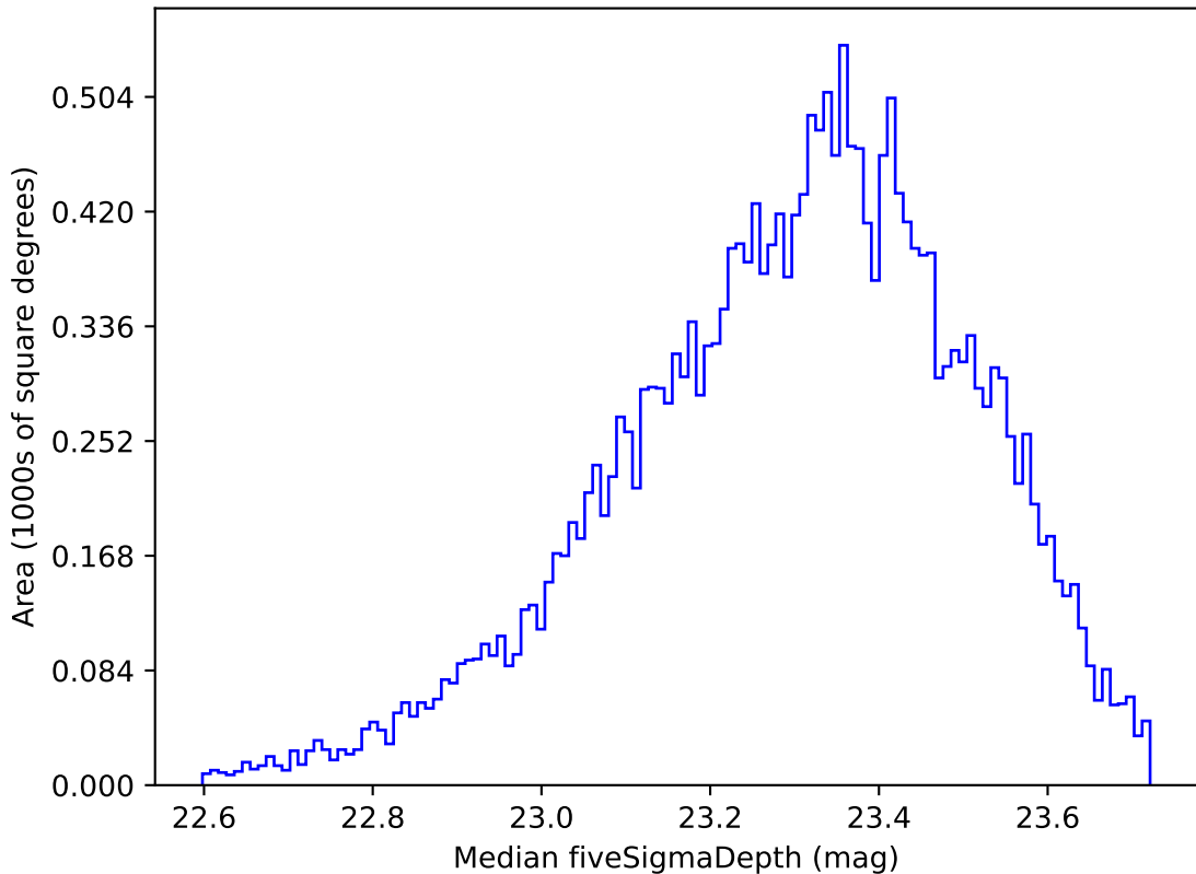
weather_cloudso30v3.4_10yrs Yr 1 u band: Median fiveSigmaDepth
