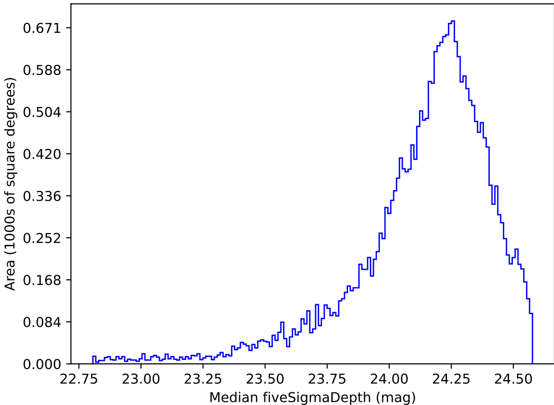
weather_cloudso30v3.4_10yrs Yr 1 r band: Median fiveSigmaDepth
