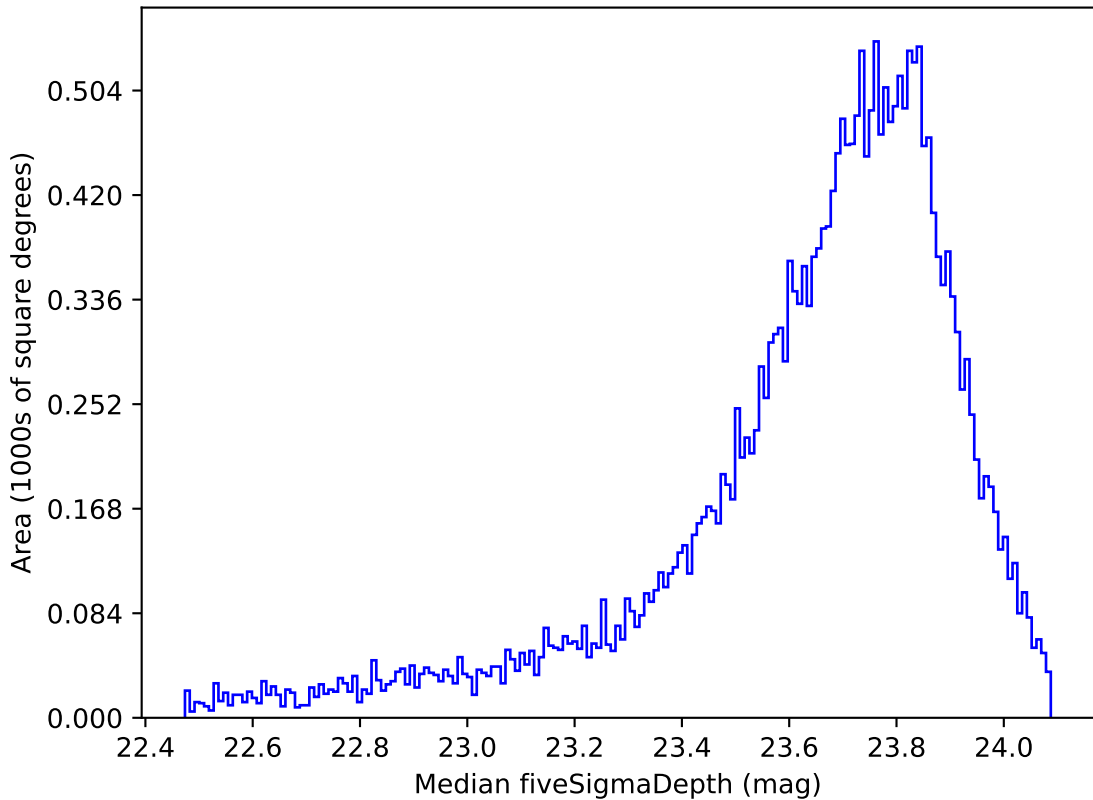
weather_cloudso30v3.4_10yrs Yr 1 i band: Median fiveSigmaDepth
