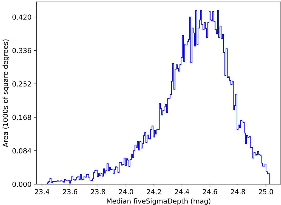
weather_cloudso3v3.4_10yrs Yr 1 g band: Median fiveSigmaDepth
