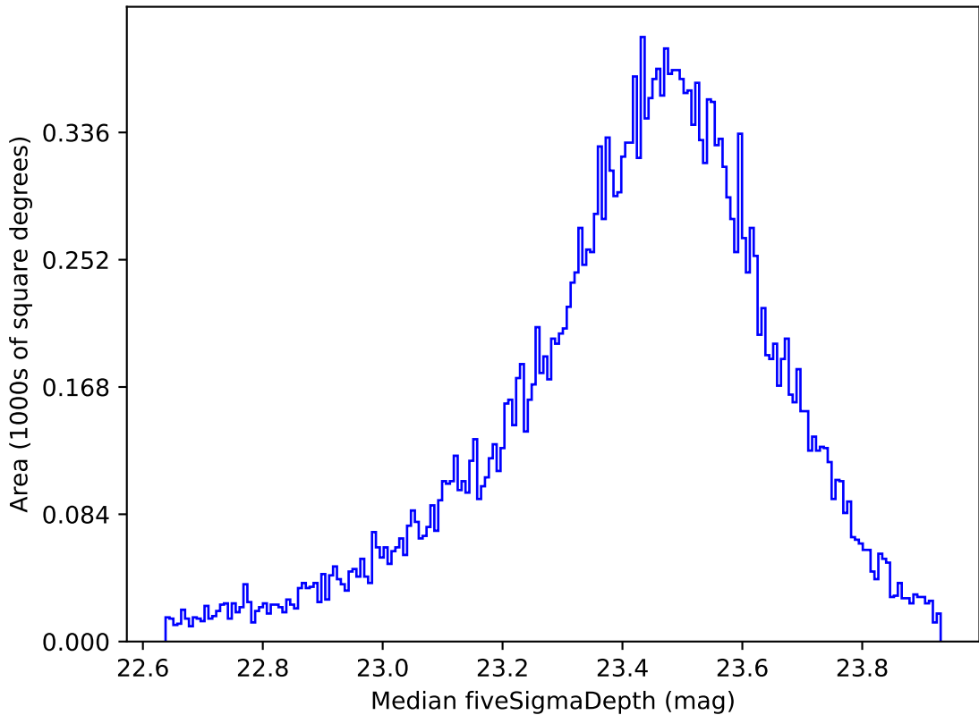
weather_cloudso30v3.4_10yrs Yr 1 all bands: Median fiveSigmaDepth
