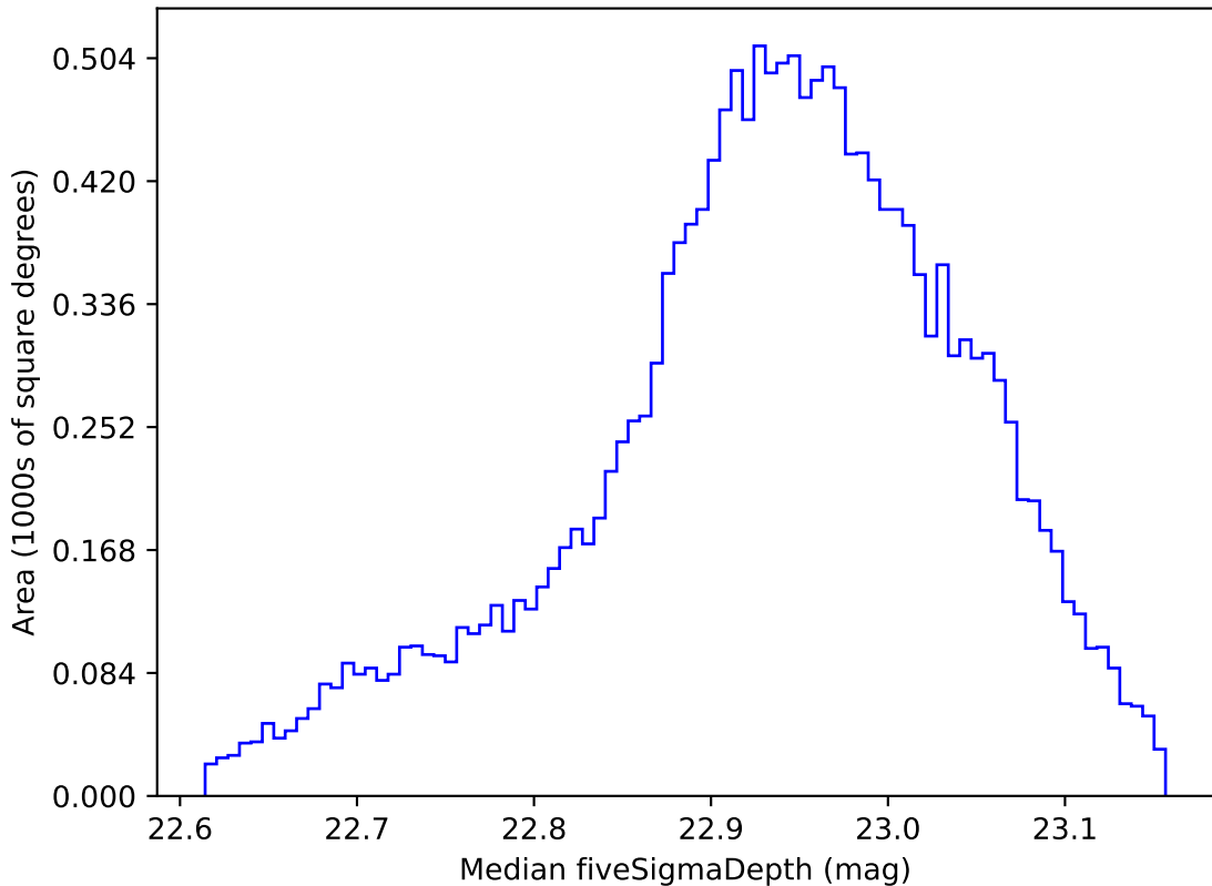
weather_cloudso30v3.4_10yrs WFD z band: Median fiveSigmaDepth
