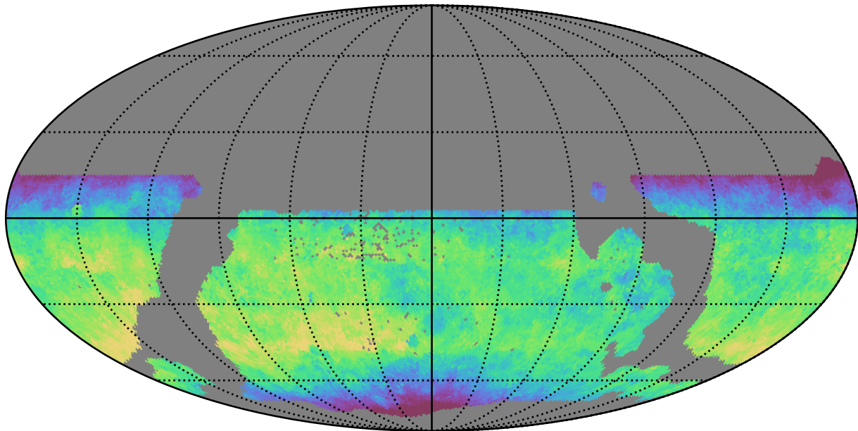
weather_cloudso30v3.4_10yrs WFD y band: Median fiveSigmaDepth
