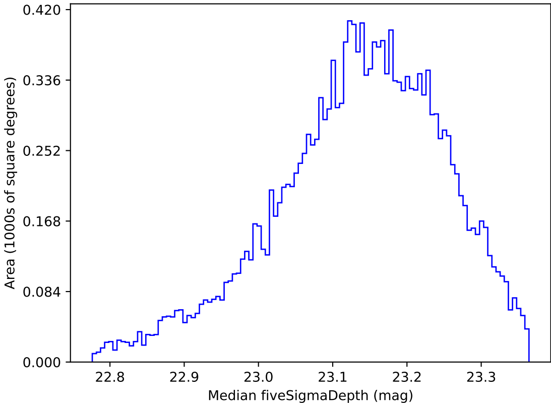
weather_cloudso30v3.4_10yrs WFD u band: Median fiveSigmaDepth
