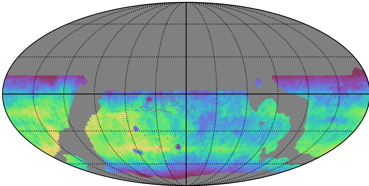
weather_cloudso30v3.4_10yrs WFD r band: Median fiveSigmaDepth
