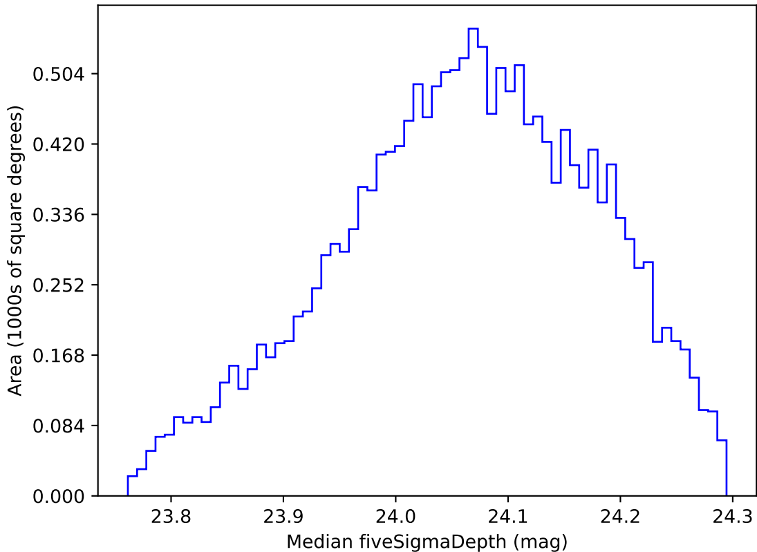
weather_cloudso30v3.4_10yrs WFD r band: Median fiveSigmaDepth
