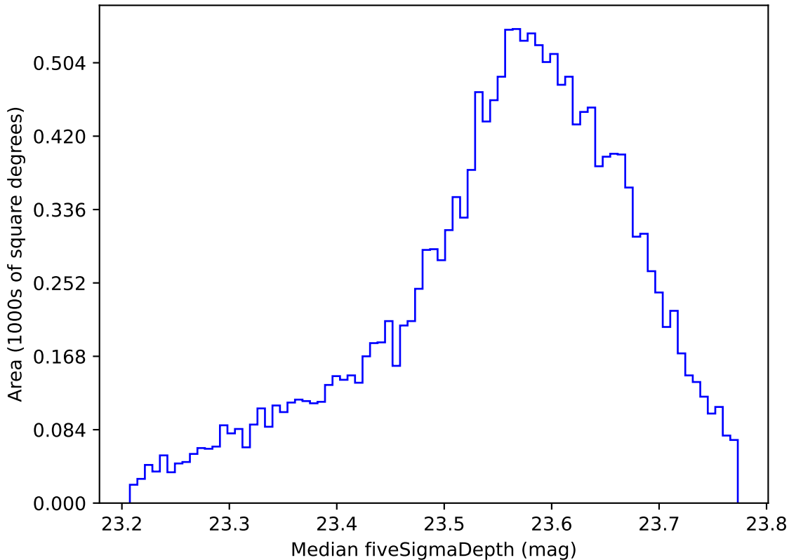
weather_cloudso30v3.4_10yrs WFD i band: Median fiveSigmaDepth
