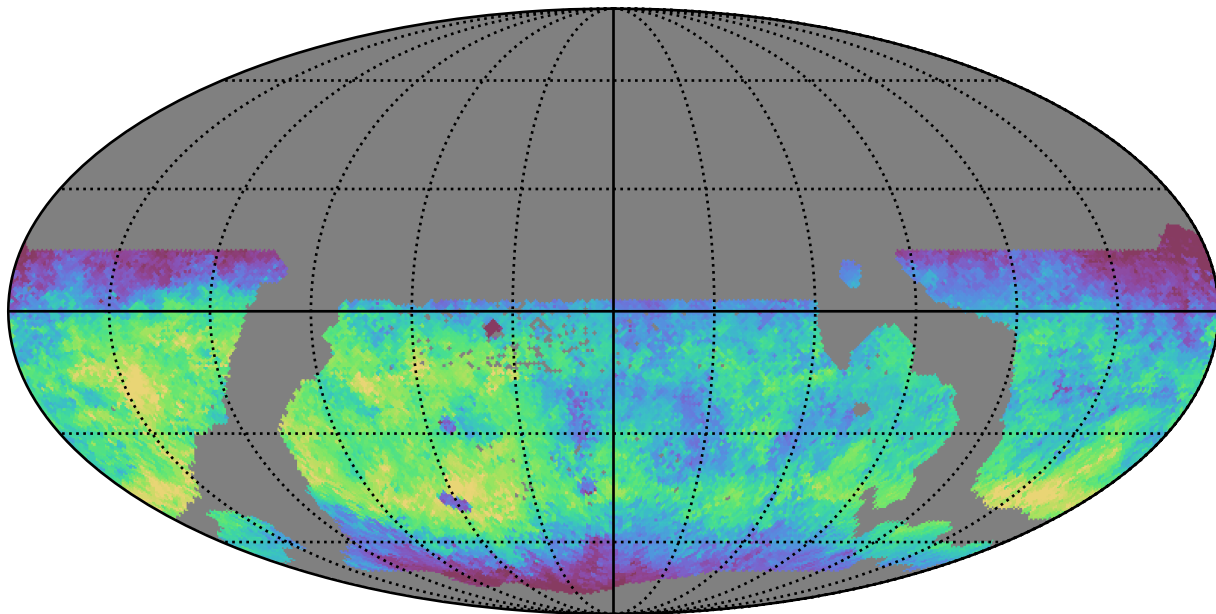
weather_cloudso30v3.4_10yrs WFD g band: Median fiveSigmaDepth
