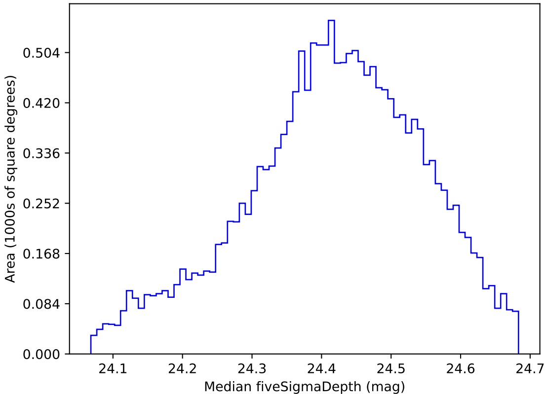
weather_cloudso30v3.4_10yrs WFD g band: Median fiveSigmaDepth
