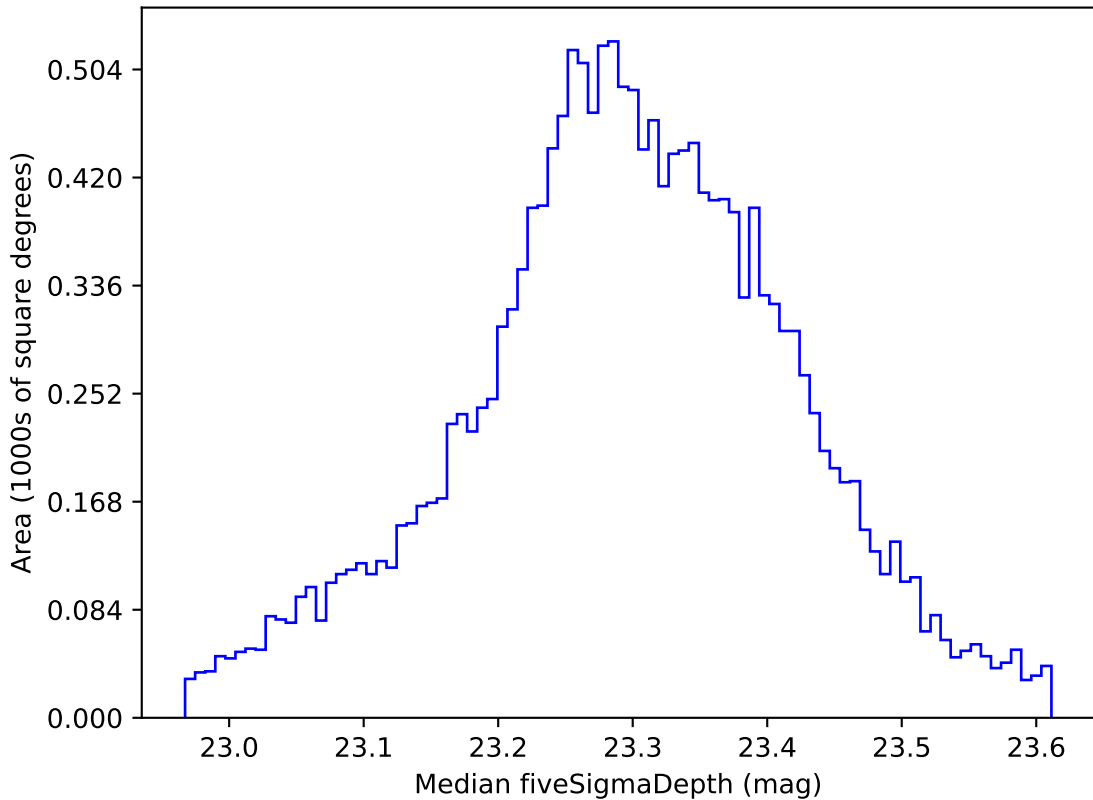
weather_cloudso30v3.4_10yrs WFD all bands: Median fiveSigmaDepth
