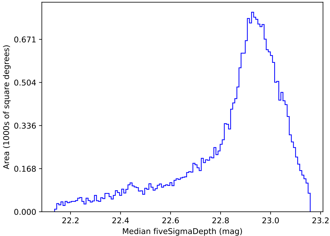
weather_cloudso30v3.4_10yrs All sky z band: Median fiveSigmaDepth
