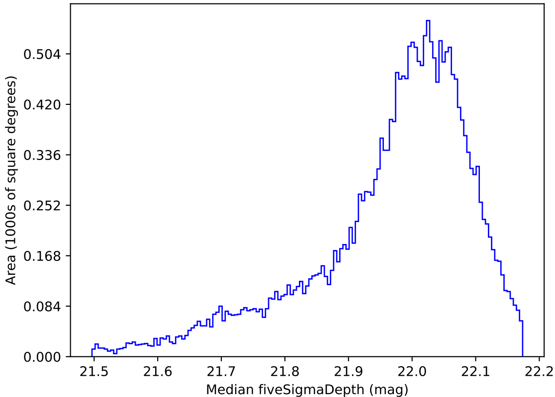
weather_cloudso30v3.4_10yrs All sky y band: Median fiveSigmaDepth
