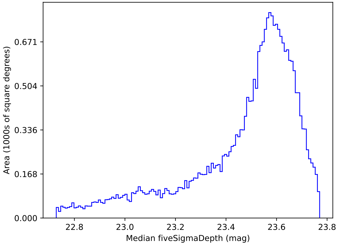
weather_cloudso30v3.4_10yrs All sky i band: Median fiveSigmaDepth
