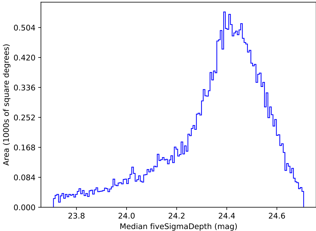
weather_cloudso30v3.4_10yrs All sky g band: Median fiveSigmaDepth
