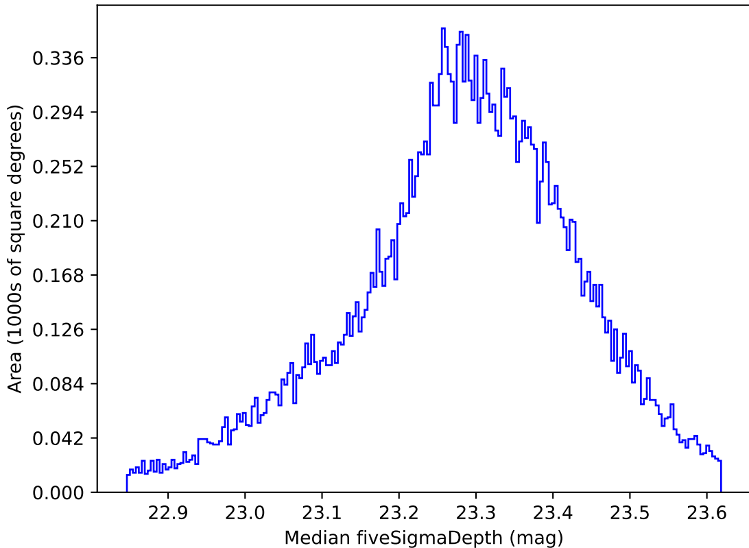
weather_cloudso30v3.4_10yrs All sky all bands: Median fiveSigmaDepth
