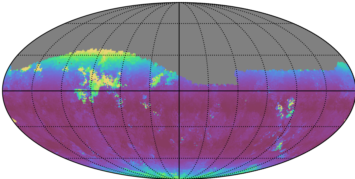
weather_cloudso30v3.4_10yrs Yr 1 z band: Median airmass
