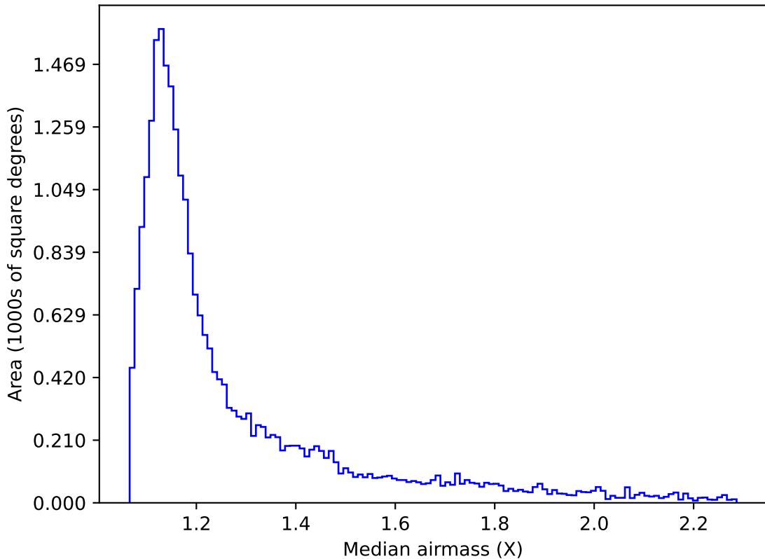
weather_cloudso30v3.4_10yrs Yr 1 z band: Median airmass
