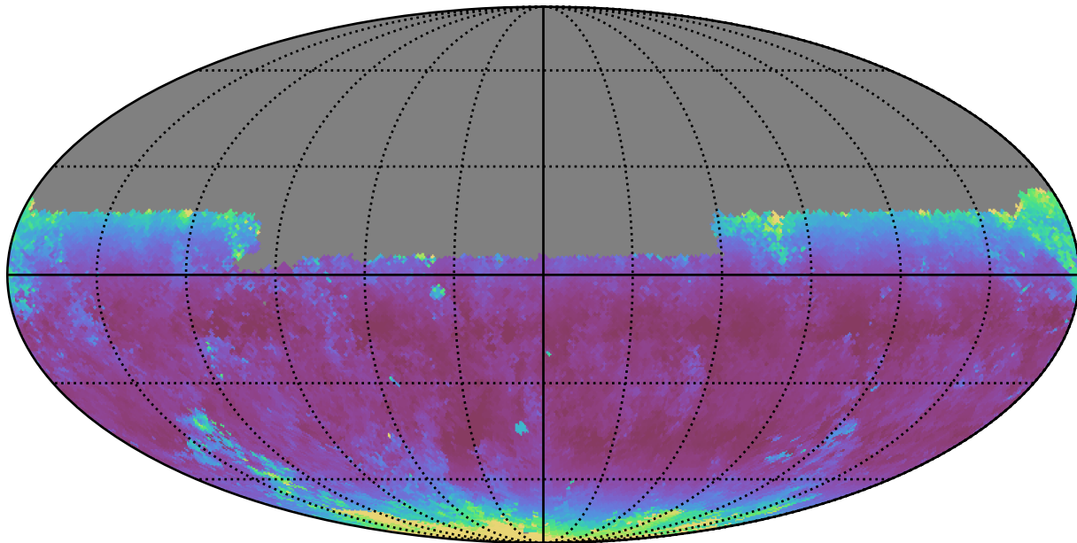
weather_cloudso30v3.4_10yrs Yr 1 y band: Median airmass
