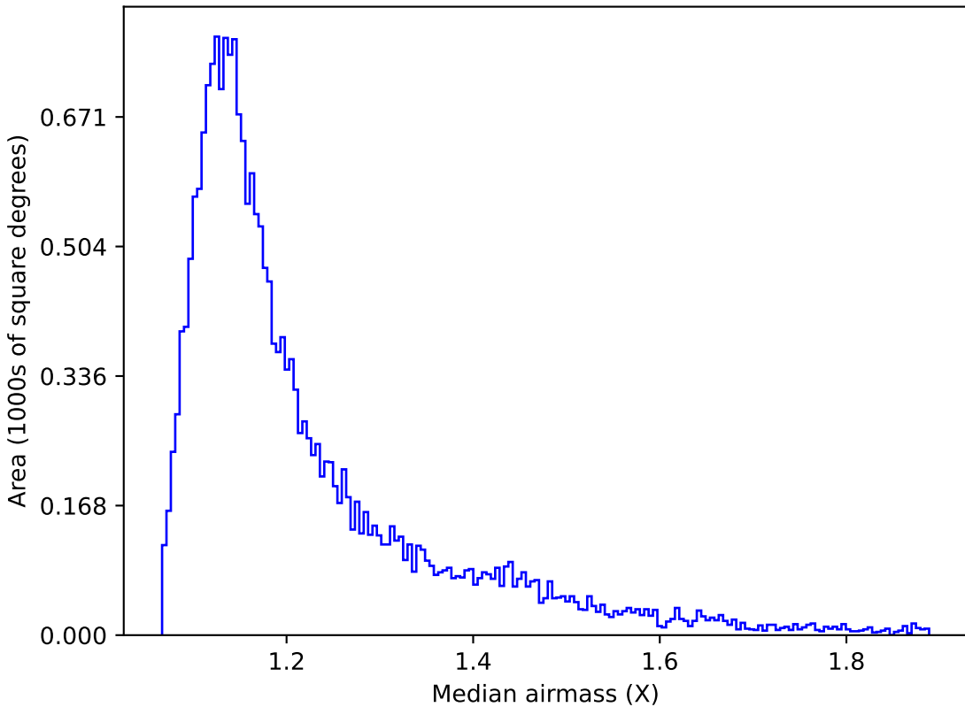
weather_cloudso30v3.4_10yrs Yr 1 y band: Median airmass
