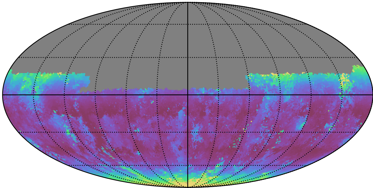
weather_cloudso30v3.4_10yrs Yr 1 u band: Median airmass
