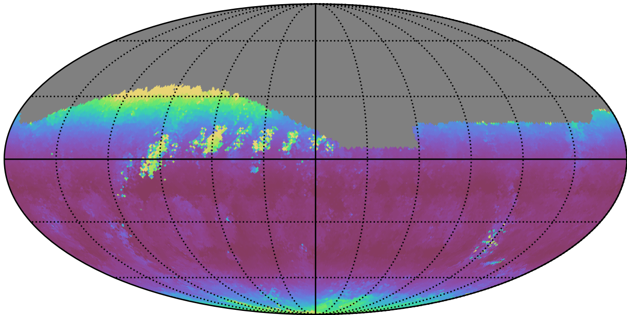
weather_cloudso30v3.4_10yrs Yr 1 r band: Median airmass
