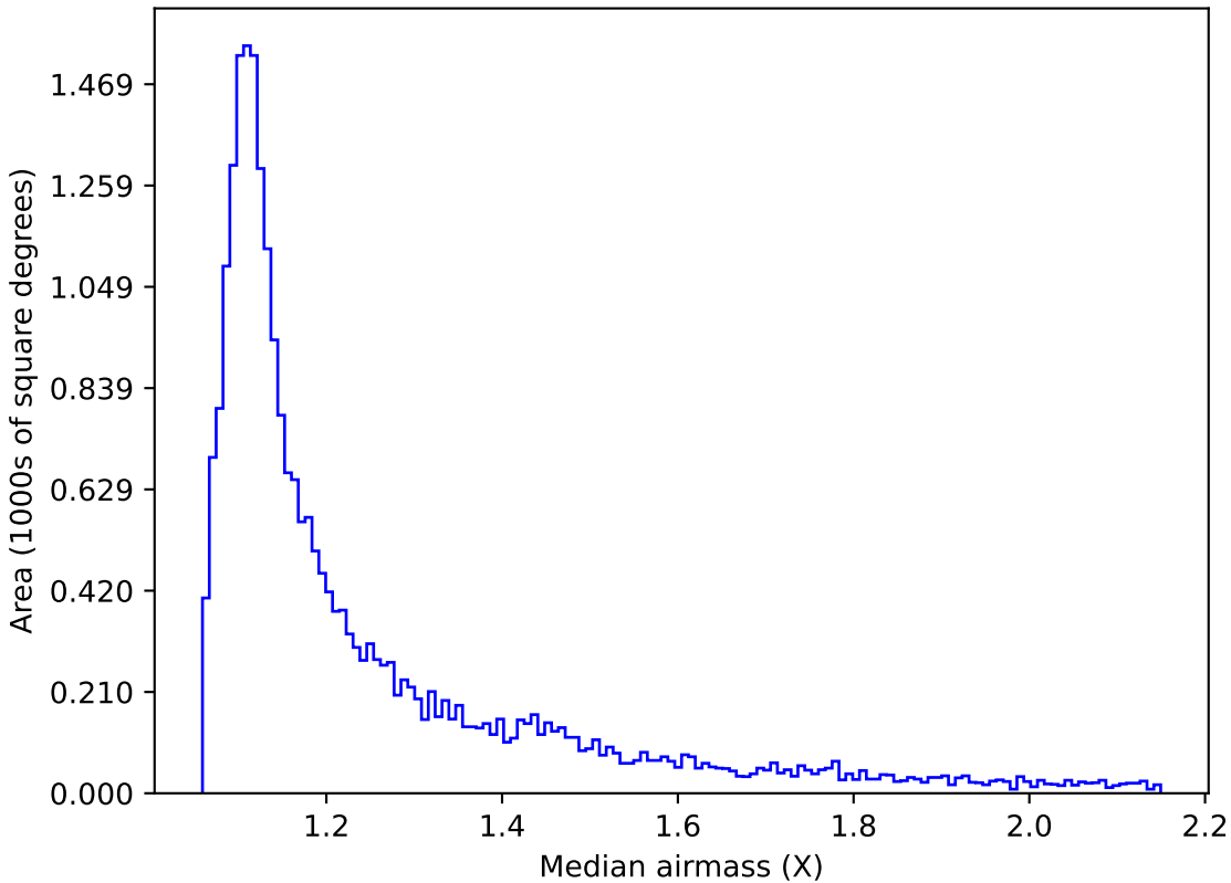
weather_cloudso30v3.4_10yrs Yr 1 r band: Median airmass
