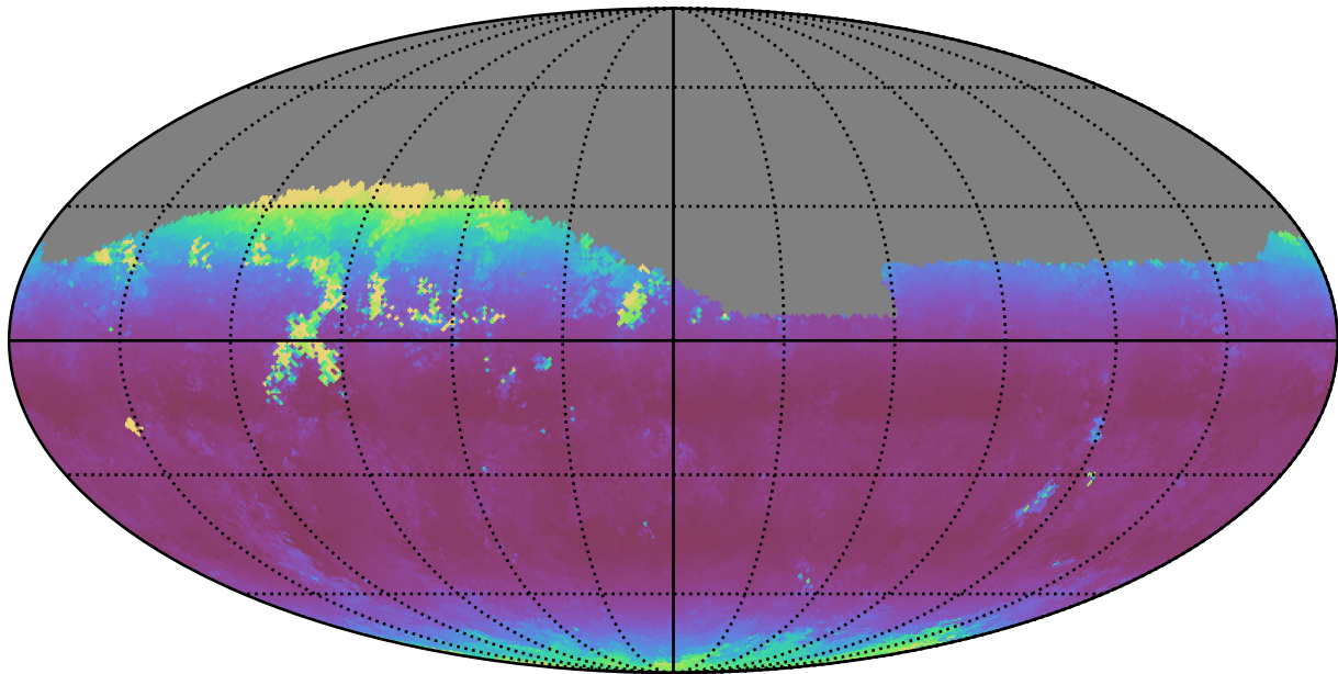
weather_cloudso30v3.4_10yrs Yr 1 i band: Median airmass
