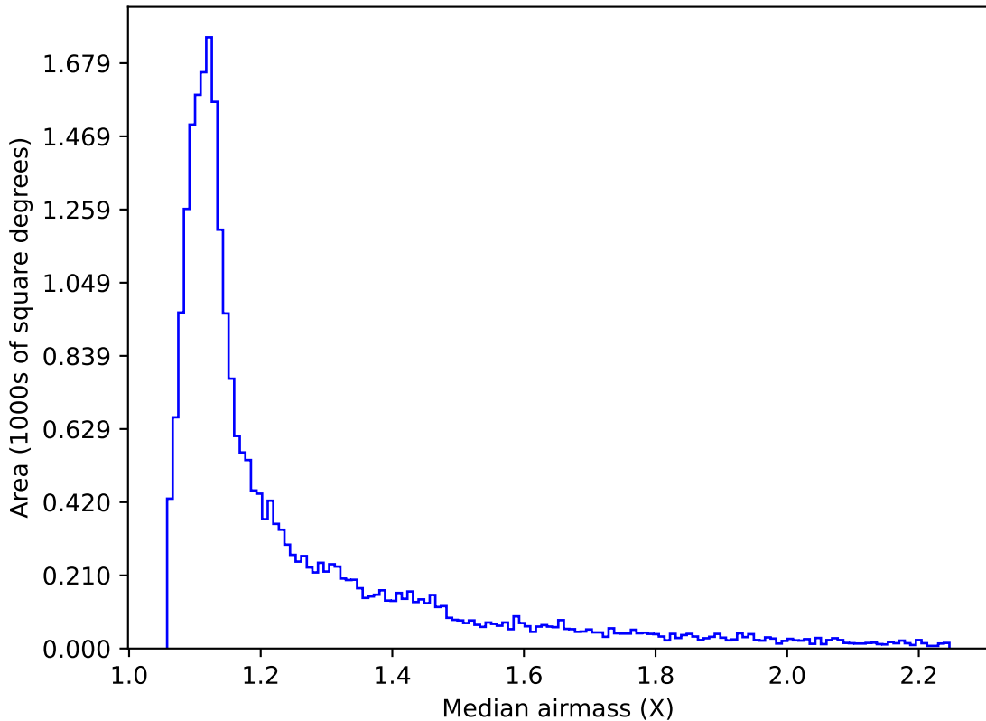
weather_cloudso30v3.4_10yrs Yr 1 i band: Median airmass
