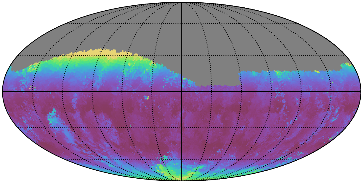
weather_cloudso30v3.4_10yrs Yr 1 g band: Median airmass
