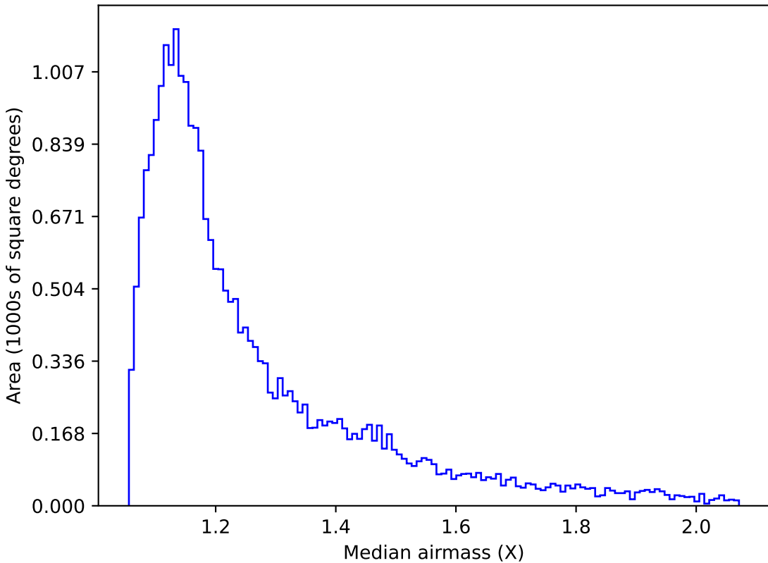
weather_cloudso30v3.4_10yrs Yr 1 g band: Median airmass
