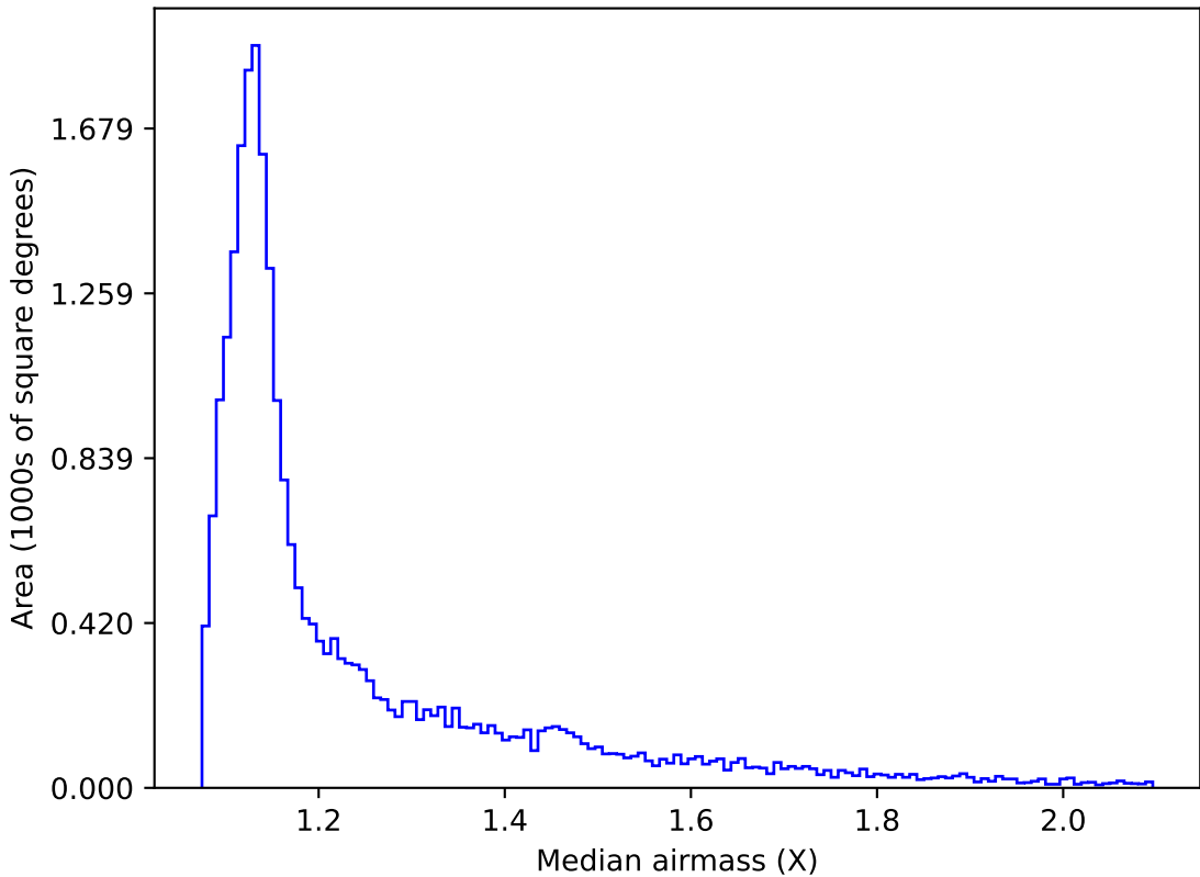
weather_cloudso30v3.4_10yrs Yr 1 all bands: Median airmass
