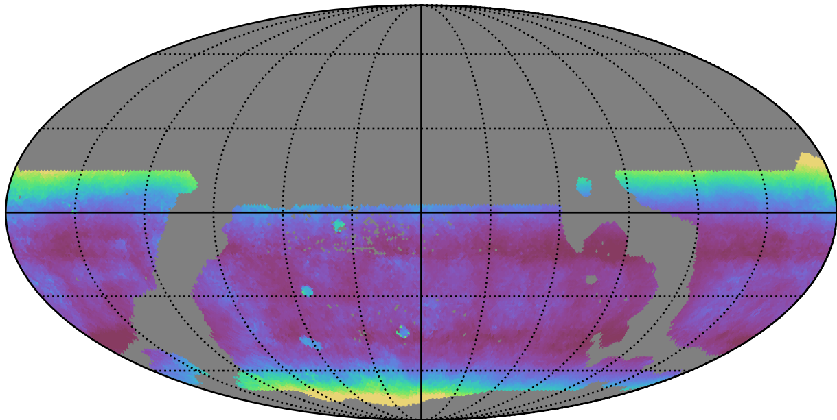
weather_cloudso30v3.4_10yrs WFD z band: Median airmass
