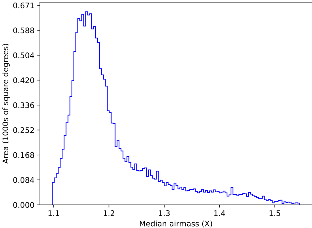
weather_cloudso30v3.4_10yrs WFD z band: Median airmass
