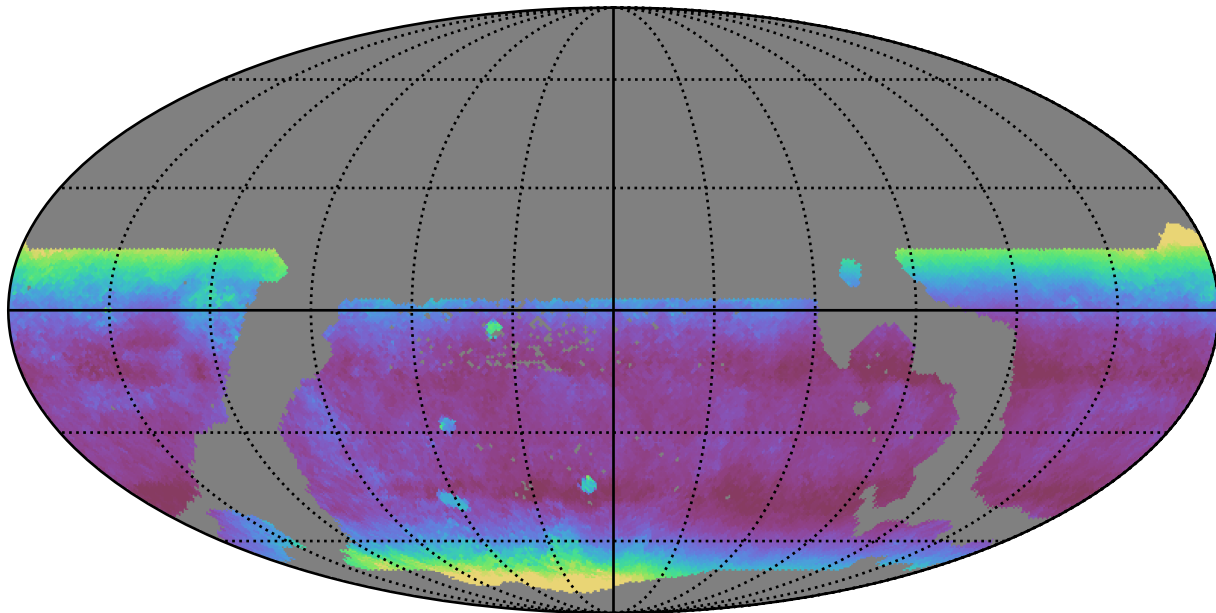
weather_cloudso30v3.4_10yrs WFD y band: Median airmass
